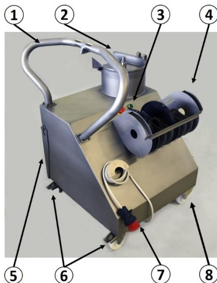
Fig. 2: Components of the basic unit
