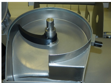
Fig. 20: Inserted ejector
