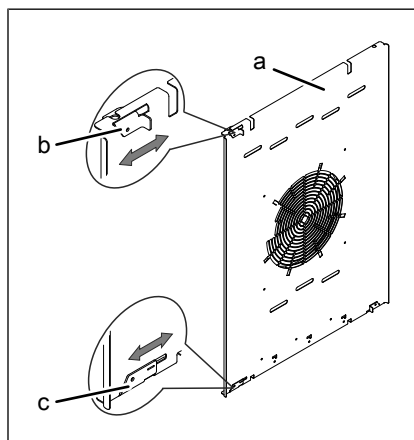
Image: Air diverter fastener
