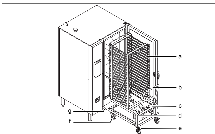
Image: Loading and emptying with a tray trolley
