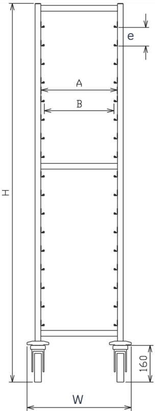
Front View
