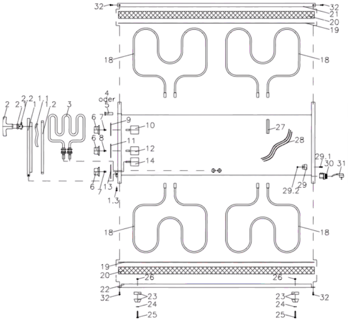
Exploded View
