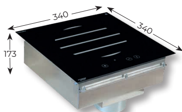
Product cut-out dimensions 346 x 346mm
